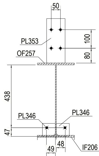
SEC A 1:10
